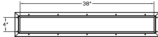
SLIMLINE PANEL GLAZING FASTENER DETAIL N.T.S.
