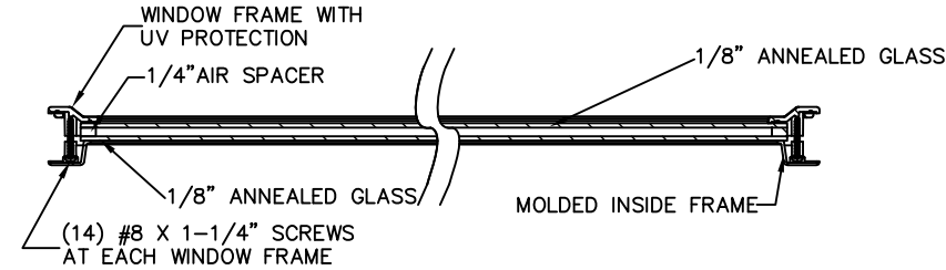
SECTION C-C
